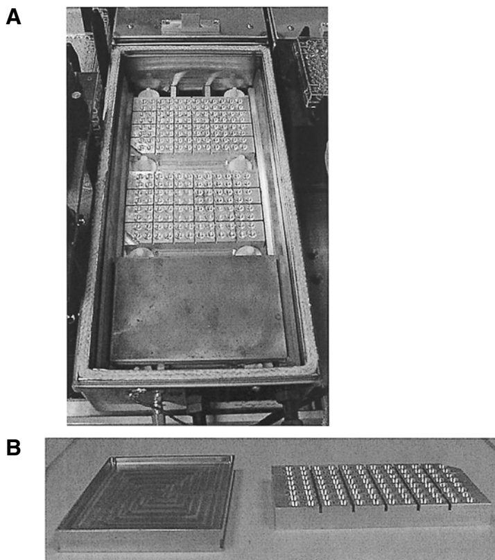
Fig. 2. Custom-modified microtiter plate incubators showing (A) brass insert guides, lid, and aluminum form-fitting inserts and (B) closeup of brass plate lid and aluminum insert. The gripper arm of the probe head moves the incubator lids and the individual brass plate lids.
